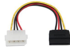
POWER ADAPTER MALE TO MALE 4-PIN MOLEX TO 15-PIN MOLEX 6"
